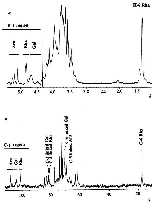
Fig. 1. ^1\text{H} (a) and ^{13}\text{C} (b) NMR spectra of arabinogalactorhamnoglycan.
